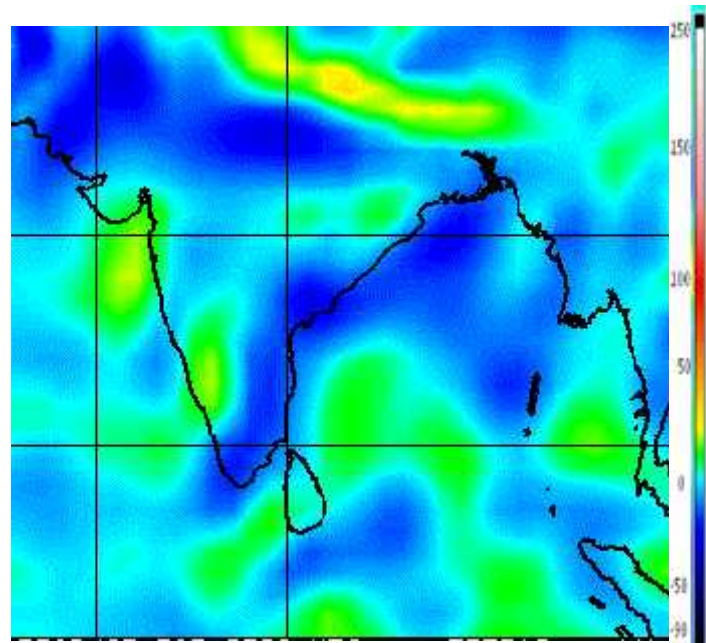
Figure B: Green yellow orange colour indicates the location of monsoon trough. (Relative vorticity map of 8:30 AM)(Source: http://cimss.ssec.wisc.edu )
