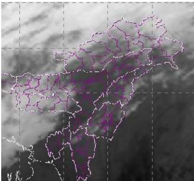
Figure A: KALPANA-1 image of 8.30 AM (white patches indicates the cloud). (Source: http://imd.gov.in )
